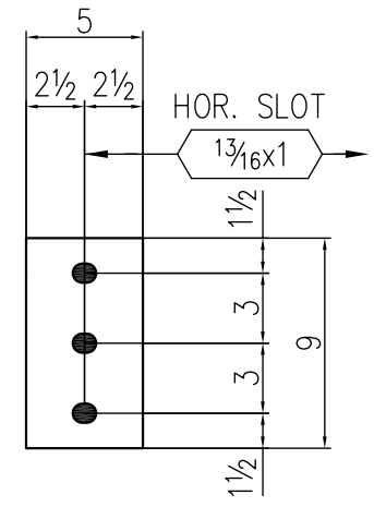
DETAIL ~ b107
