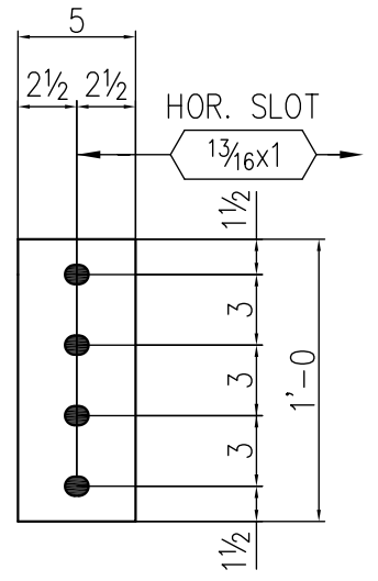
DETAIL ~ b108
