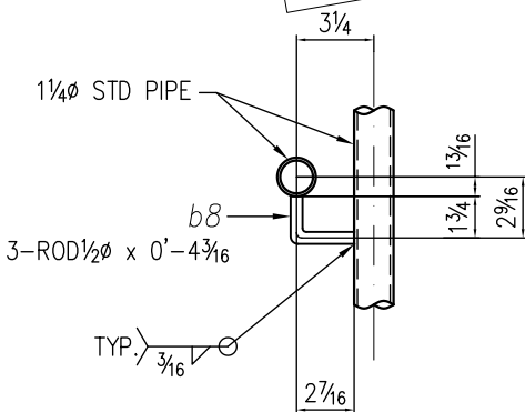
TYP. GRABRAIL BRACKET
