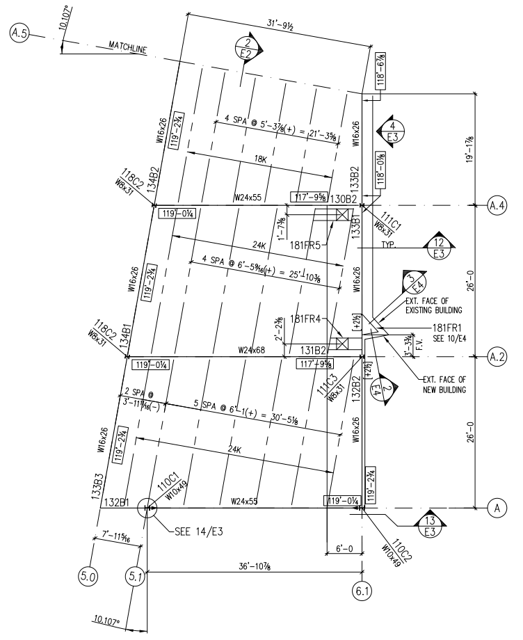
PARTIAL ROOF STEEL ERECTION PLAN 3/32"=1'-0" REF. S1.0
